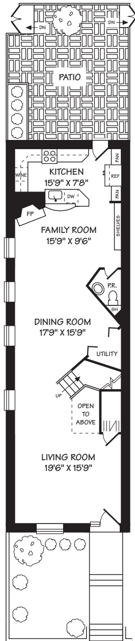
MAIN LEVEL 9' CEILING
