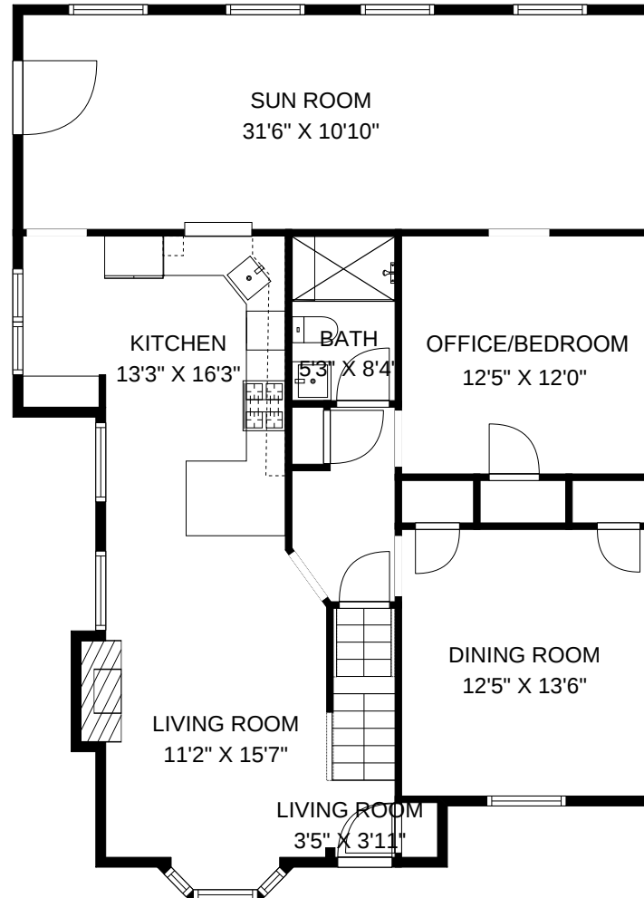
SECOND FLOOR
