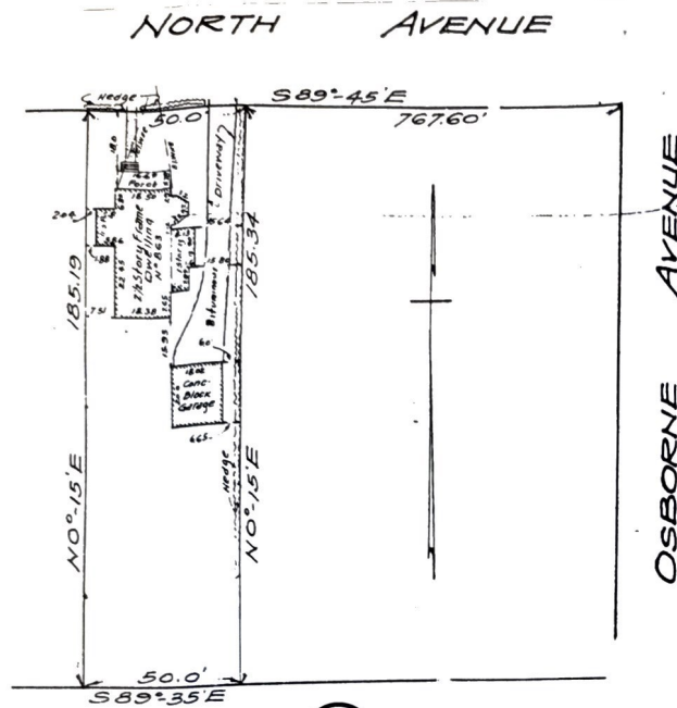
101 EXISTING SITE PLAN SCALE: 1" = 30'-0"
