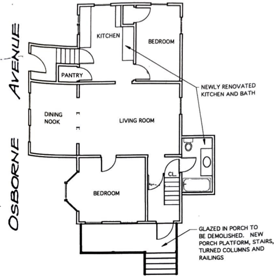
102 EXISTING 1ST FLOOR PLAN SCALE: 1/8" = 1'-0"
