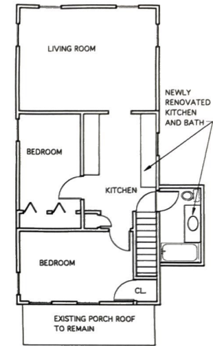
103 EXISTING 2ND FLOOR PLAN SCALE: 1/8" = 1'-0"
